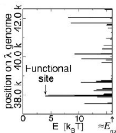
Figure 6 Energy landscape for the TF Cro on the bacteriophage \lambda DNA(Gerland et al., 2002). The landscape appears to be random, with different strength.
