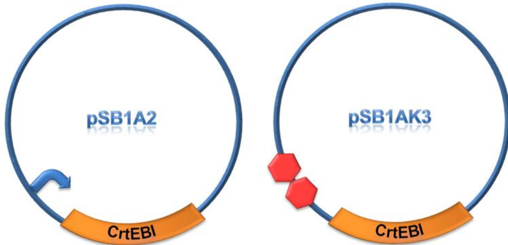
Figure 1 Biobricks we constructed to characterize biobrick BBa_K274100. The left construct denotes Constitutive promoter BBa_J23103-CrtEBI and on the right is an interesting biobrick—Terminator BBa_B0015-CrtEBI, namely a terminator was prefixed to CrtEBI, expected to reduce the leaky expression.
