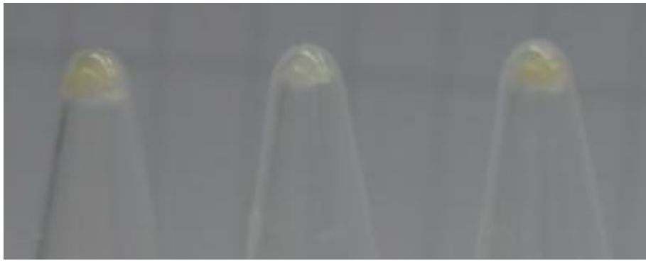
Fig 3. Color contrast after 12 hours' cultivation (for each photo, from the left to the right are JM109, BL21 and DH5 \alpha ).
