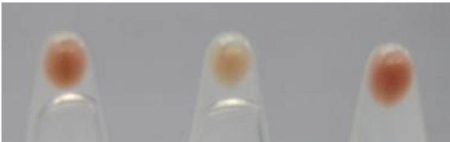
Constitutive promoter BBa_J23103-CrtEBI
